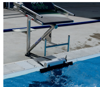
4. Wedge automatically retracts out of the water
