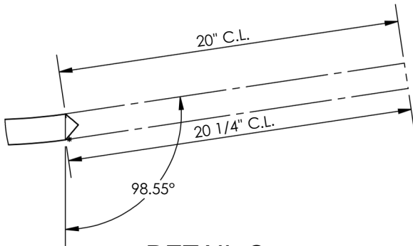
DETAIL C SCALE 1 : 8
