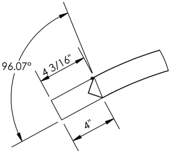
DETAIL B SCALE 1 : 8
