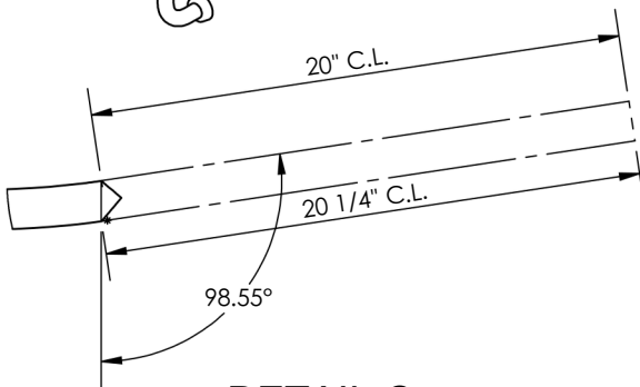
DETAIL C SCALE 1 : 8
