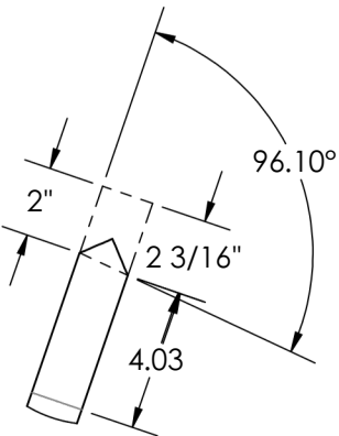
DETAIL C SCALE 1 : 6
